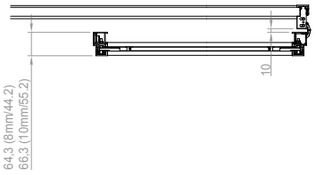
Divina single swing door open position
