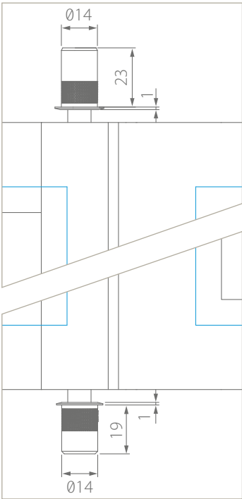
Floor sleeve and ceiling sleeve for Divina double hinged door
