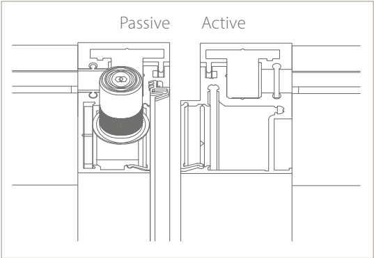
Floor sleeve and ceiling sleeve for Divina double hinged door
