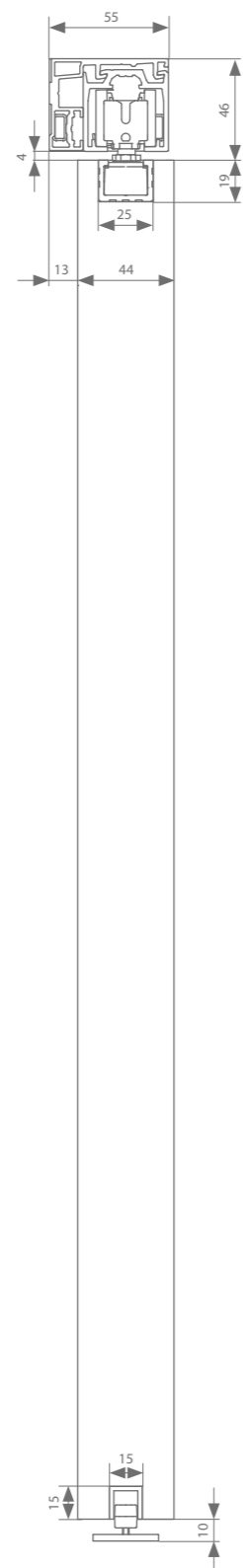
Wall mount 44 mm
