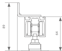
Wall mount 50 mm
