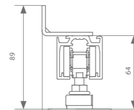
Wall mount 54 mm
