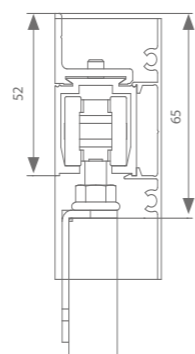
Option 2 - Version C
