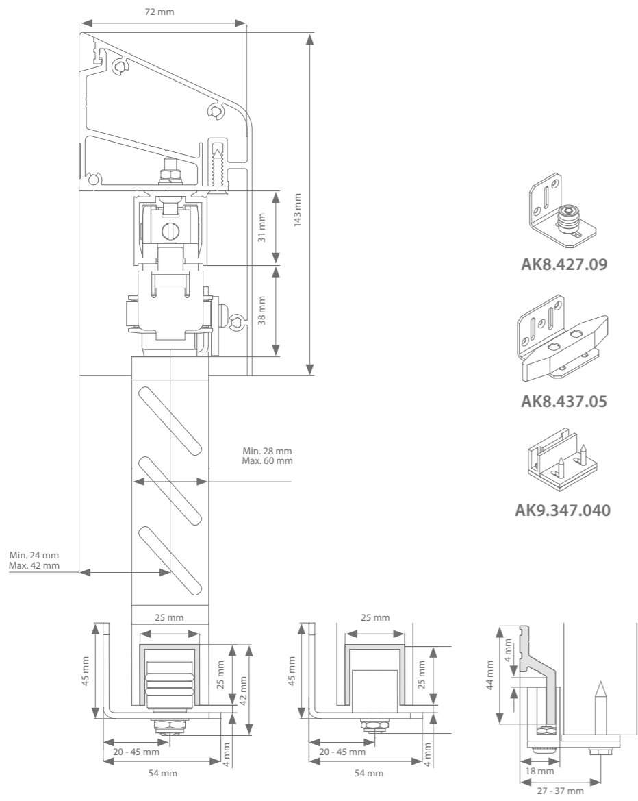
Option 1 - AK8.427.09
