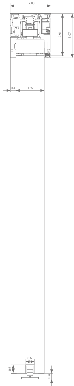
Wall mount 1.97"
