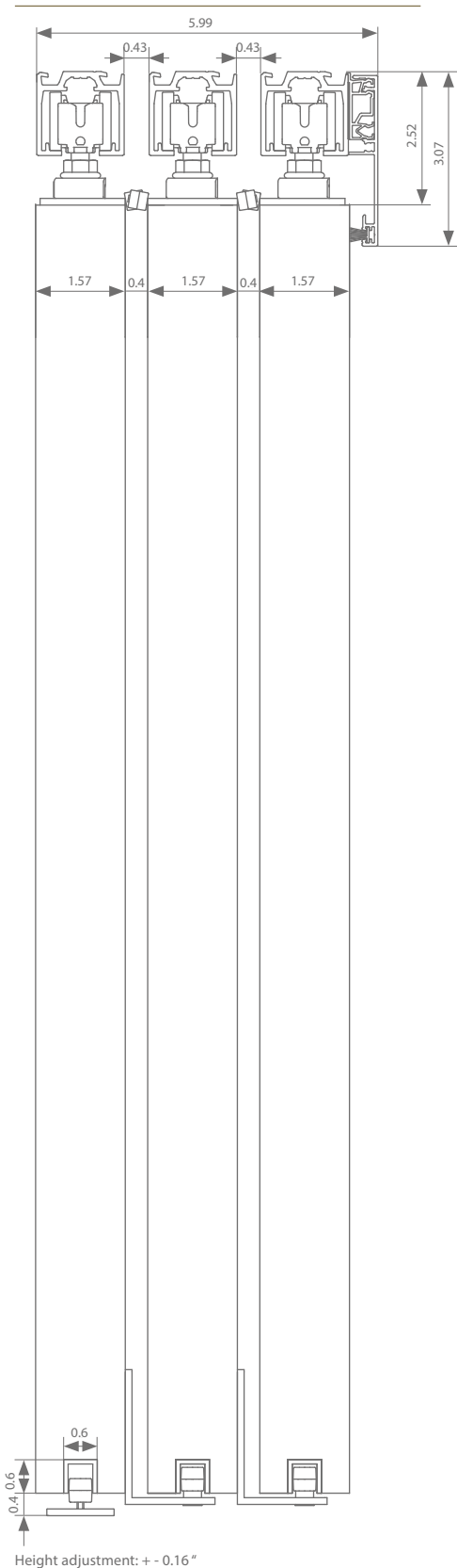
Parallel ceiling mount 1
