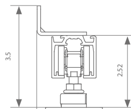
Wall mount 1.97"
