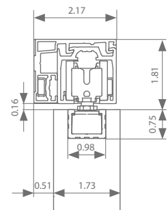
Wall mount 1.73"
