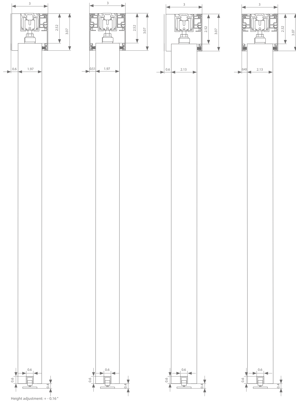
Ceiling mount 1.97"
