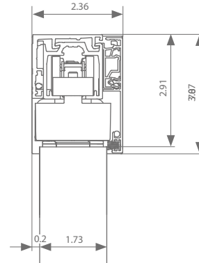
Wall mount 1.73"
