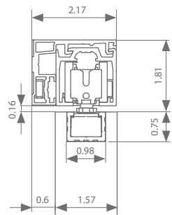
Wall mount 1.57"
