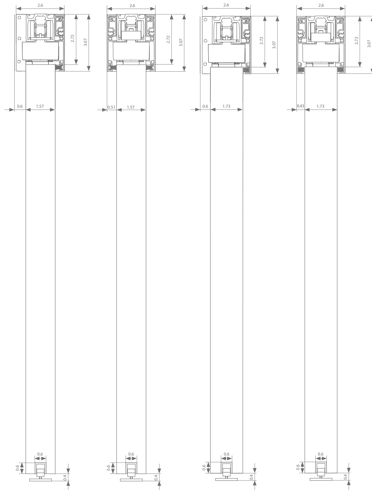
Ceiling mount 1.57"
