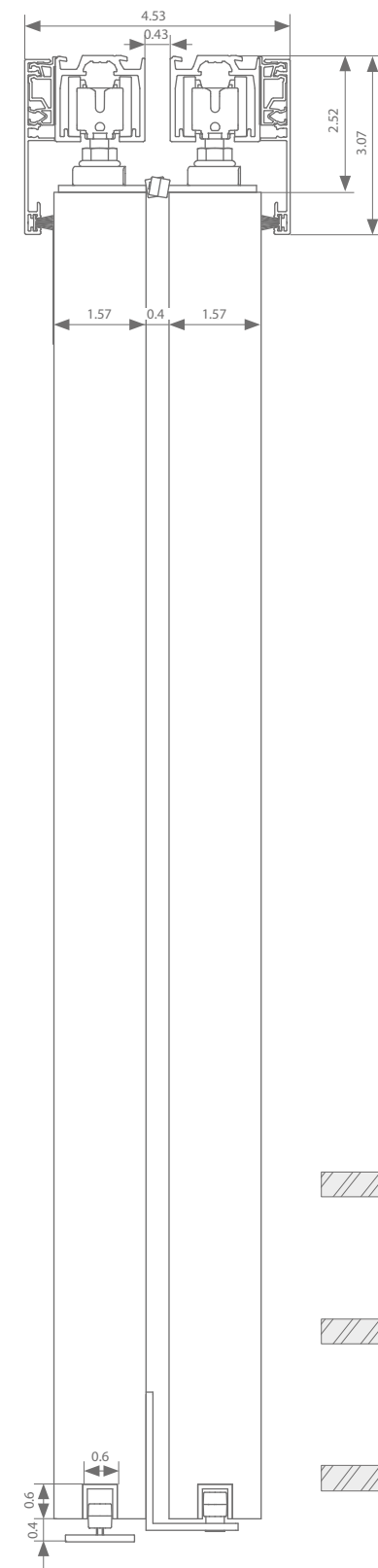
Parallel ceiling mount 2
