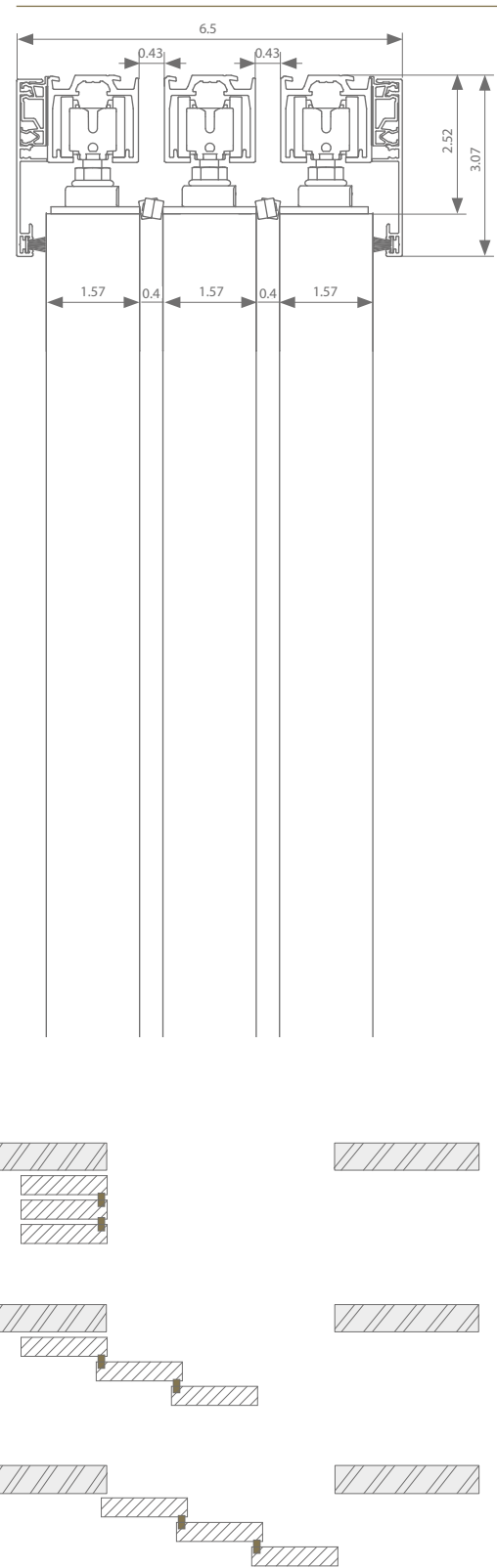
Parallel ceiling mount 2
