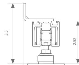
Wall mount 2.13"
