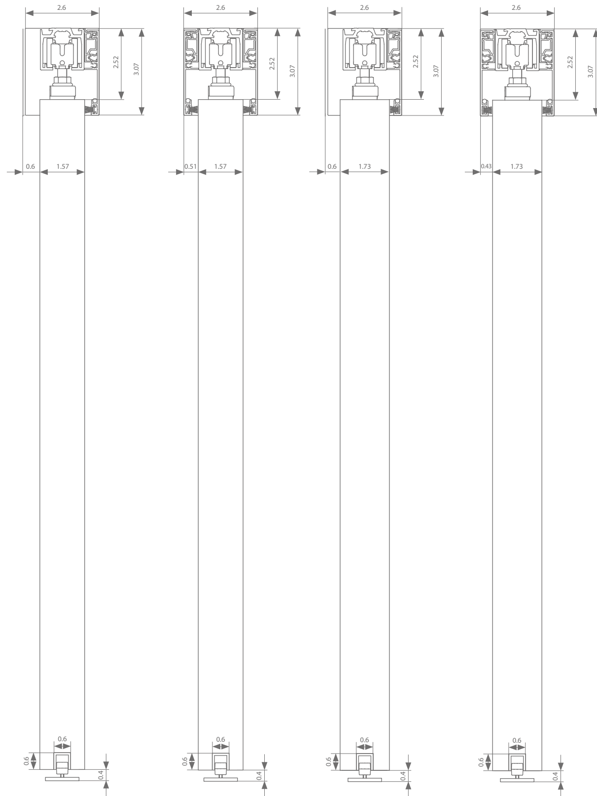
Ceiling mount 1.57"
