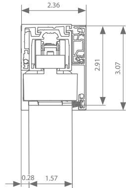
Wall mount 1.57"
