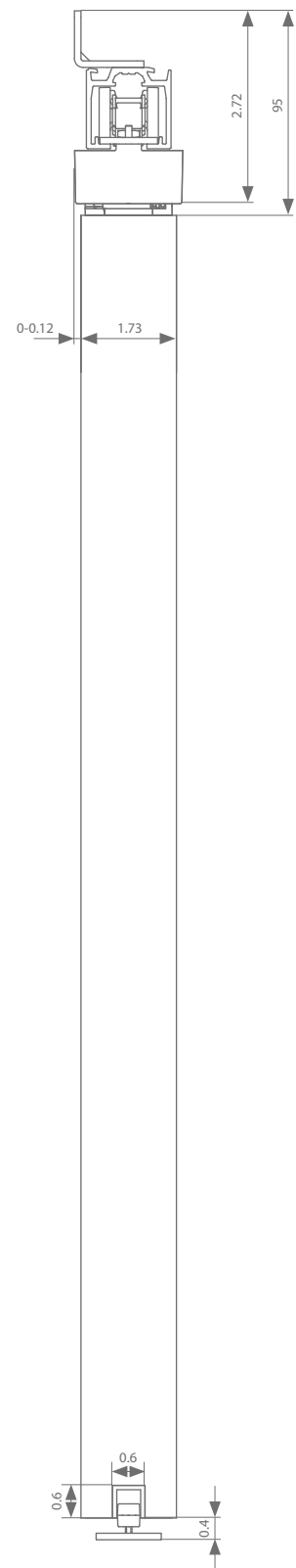
Wall mount 1.73"
