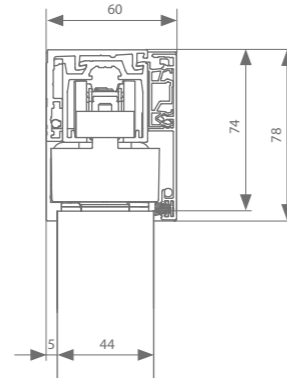
Wall mount 44 mm
