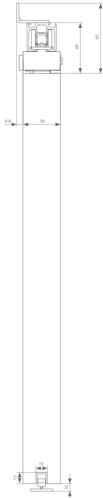
Wall mount 50 mm
