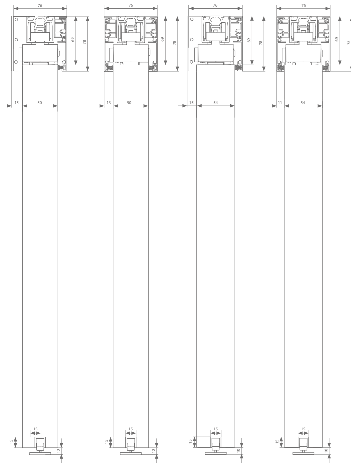
Ceiling mount 50 mm
