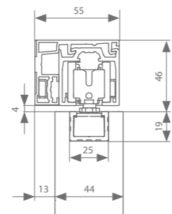
Wall mount 44 mm
