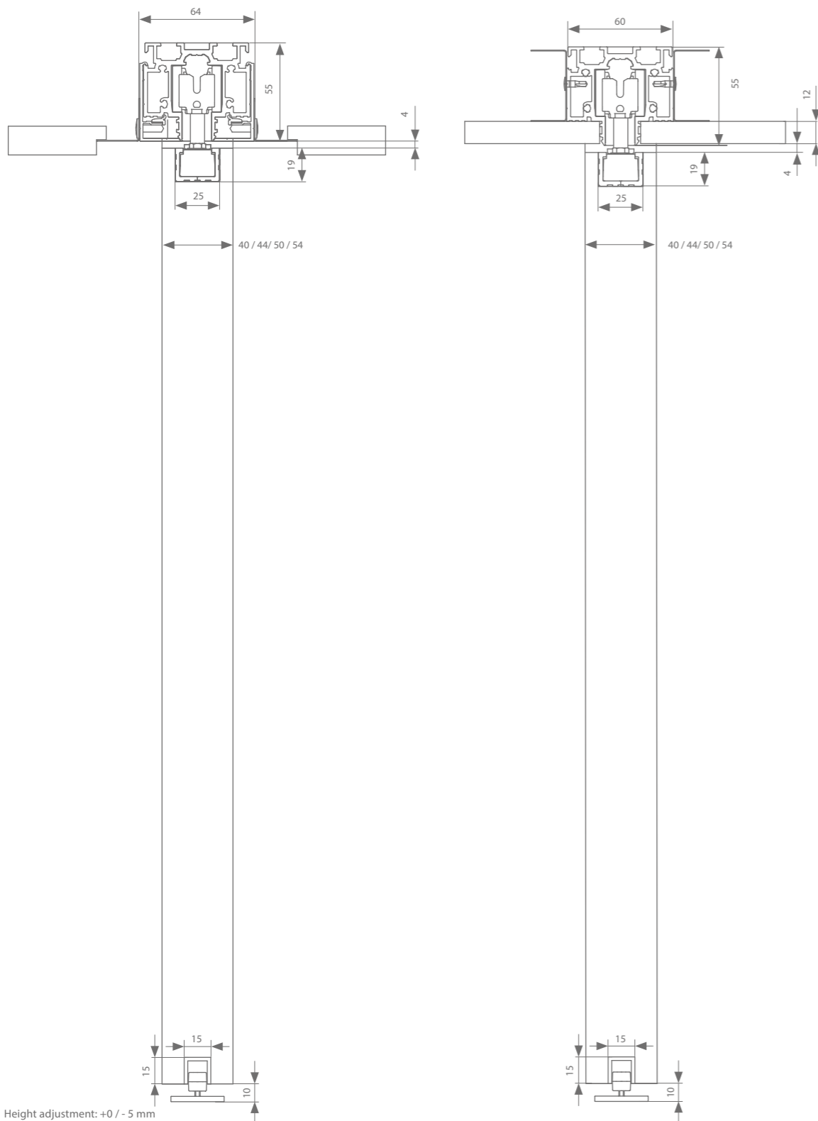
For suspended ceiling (1+2)
