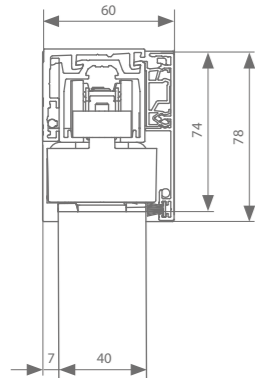
Wall mount 40 mm
