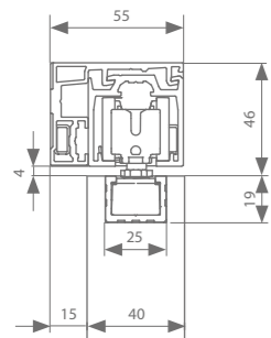
Wall mount 40 mm
