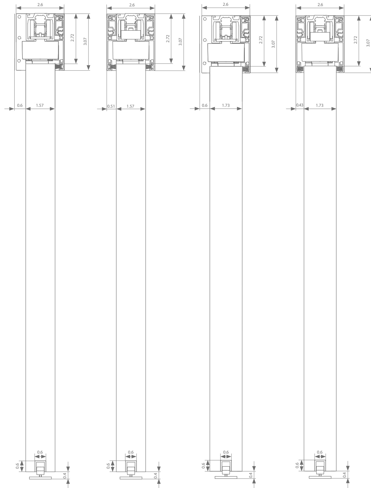
Ceiling mount 1.57"
