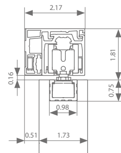
Wall mount 1.73"
