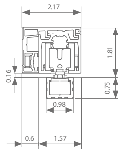
Wall mount 1.57"
